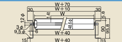
TRC-4812
